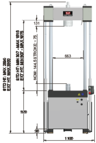
Total frame footprint 1.2 m 2 Instron 8802 Actuator in Base Dimensions All dimension are in mm
